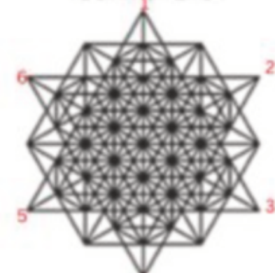
64 Tetrahedron
