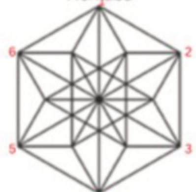
Vector Equilibrium
