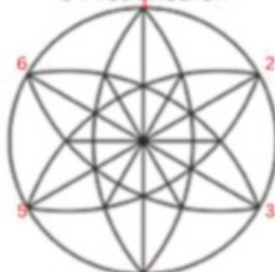
Vector Equilibrium
